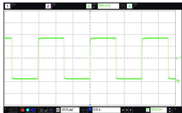
Figure 14. LVC MOS Output Waveform ( V_{\text{swing}} = 1.8\text{V} , SiT1552AI-JE-DCC-32.768, 10 pF Load)
